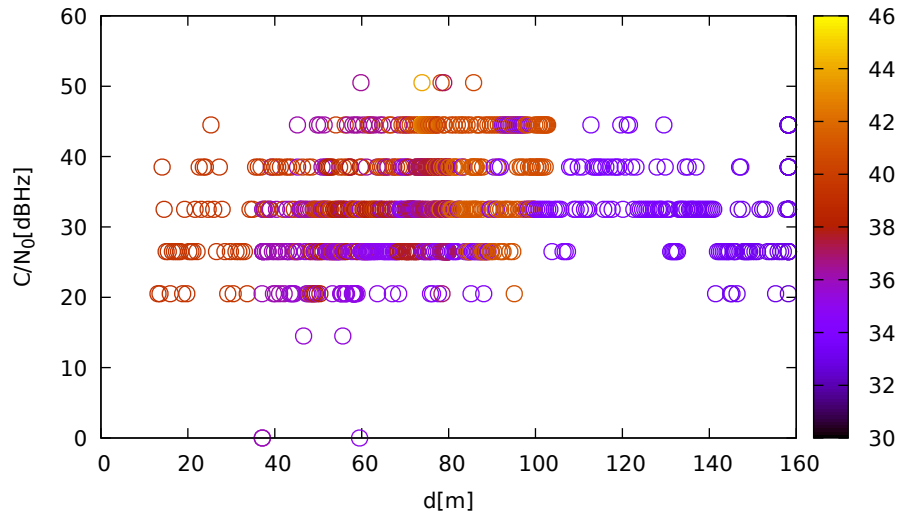
C/N 0 vs distance (LeicaGS15 at C 2 for R06 at L1)
