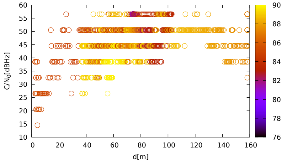
C/N 0 vs distance (LeicaGS15 at C 2 for R07 at L1)
