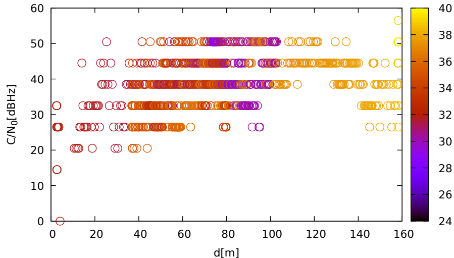
C/N 0 vs distance (LeicaGS15 at C 2 for R08 at L1)
