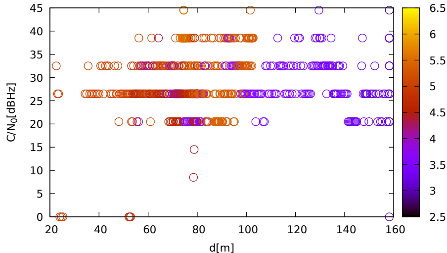
C/N 0 vs distance (LeicaGS15 at C 2 for R14 at L1)
