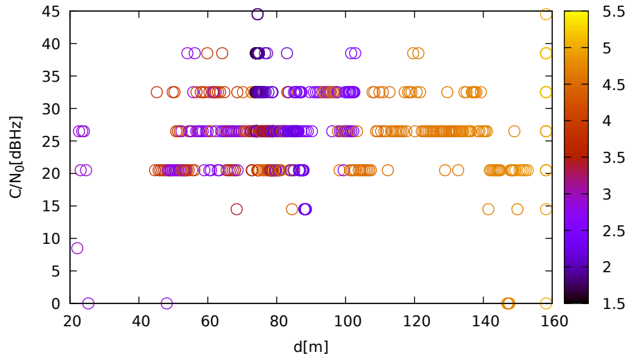
C/N 0 vs distance (LeicaGS15 at C 2 for R15 at L1)
