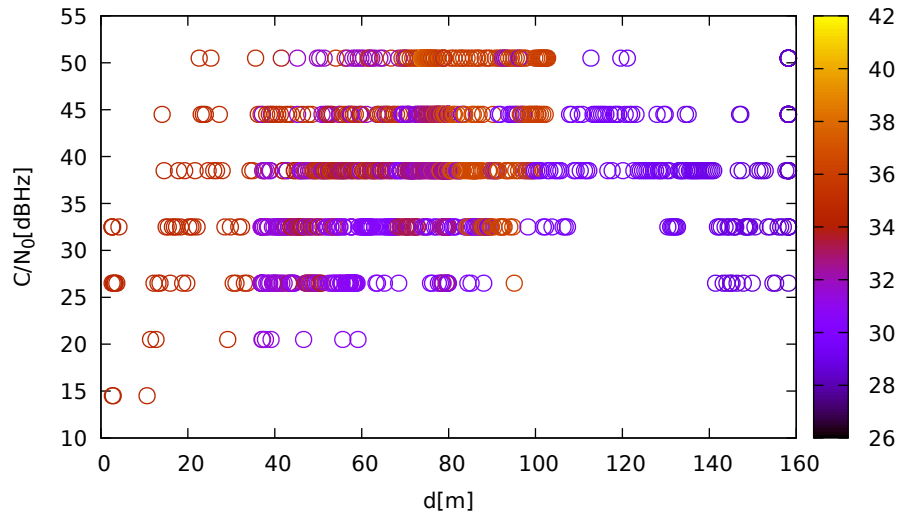
C/N 0 vs distance (LeicaGS15 at C 2 for R21 at L1)
