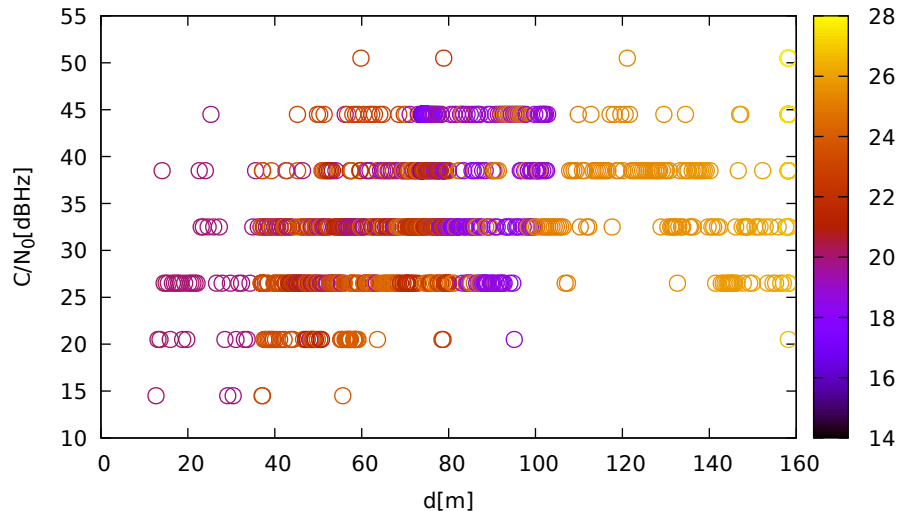
C/N 0 vs distance (LeicaGS15 at C 2 for R23 at L1)
