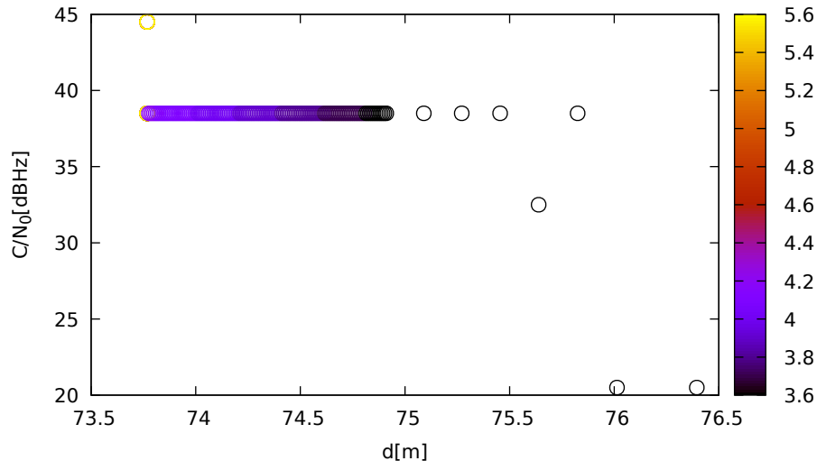
C/N 0 vs distance (LeicaGS18 at C 2 for E02 at L1)
