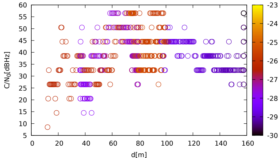
C/N 0 vs distance (LeicaGS18 at C 2 for E04 at L1)
