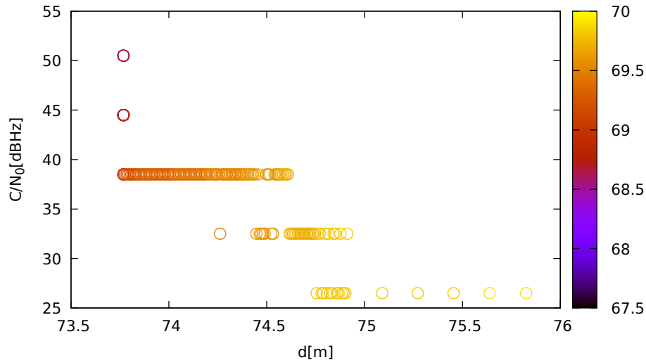
C/N 0 vs distance (LeicaGS18 at C 2 for E05 at L1)
