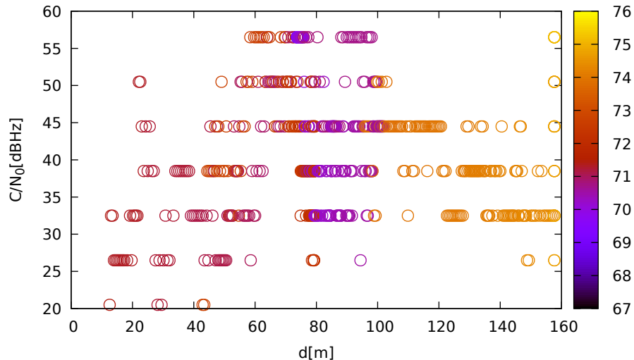
C/N 0 vs distance (LeicaGS18 at C 2 for E09 at L1)
