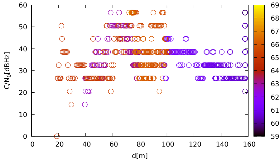
C/N 0 vs distance (LeicaGS18 at C 2 for E11 at L1)
