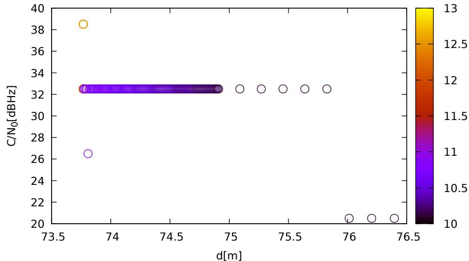
C/N 0 vs distance (LeicaGS18 at C 2 for E19 at L1)
