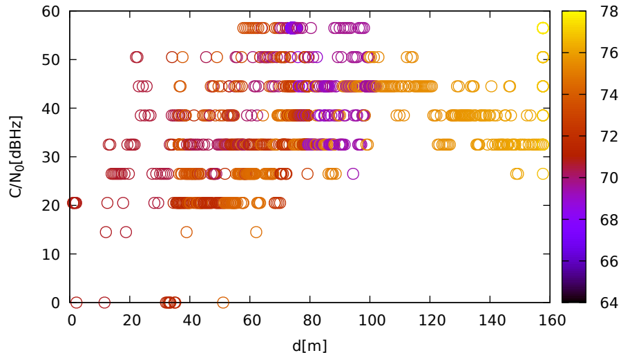
C/N 0 vs distance (LeicaGS18 at C 2 for G01 at L1)
