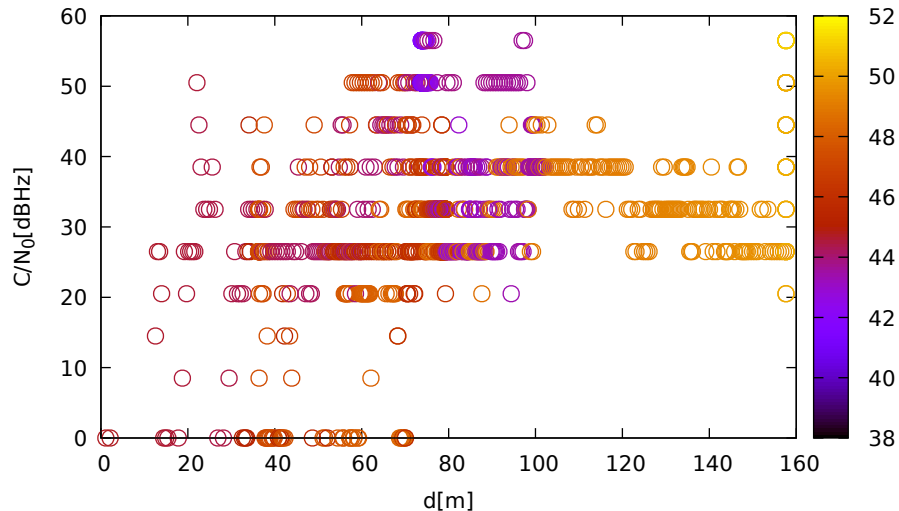
C/N 0 vs distance (LeicaGS18 at C 2 for G03 at L1)
