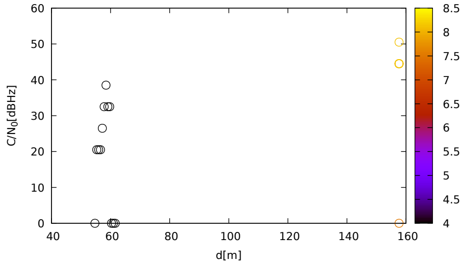
C/N 0 vs distance (LeicaGS18 at C 2 for G04 at L1)
