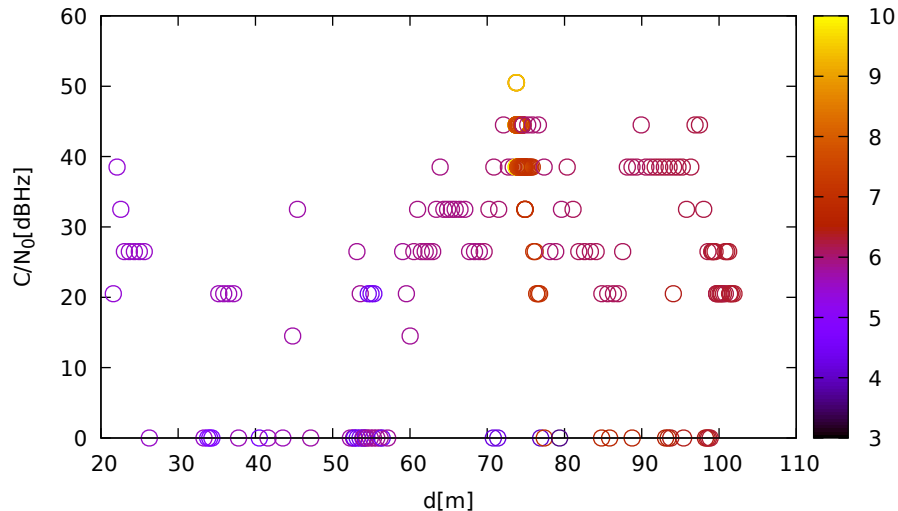
C/N 0 vs distance (LeicaGS18 at C 2 for G10 at L1)
