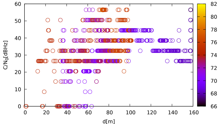
C/N 0 vs distance (LeicaGS18 at C 2 for G11 at L1)
