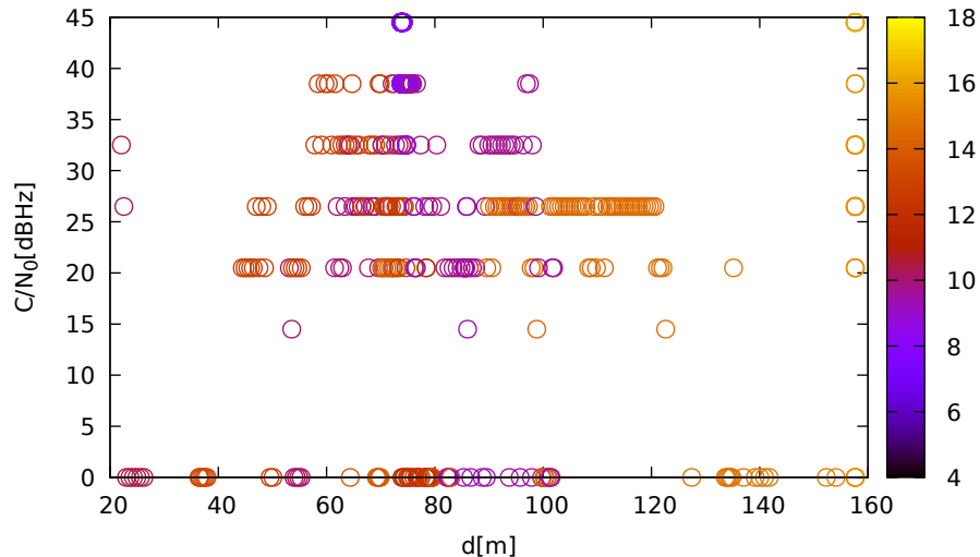
C/N 0 vs distance (LeicaGS18 at C 2 for G17 at L1)
