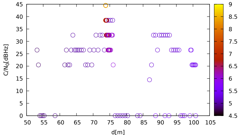
C/N 0 vs distance (LeicaGS18 at C 2 for G21 at L1)
