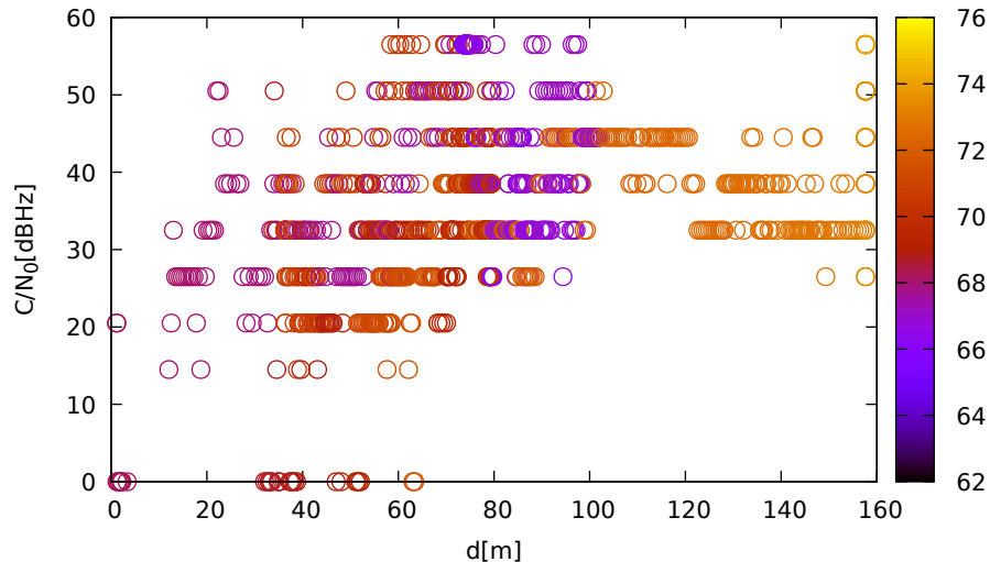
C/N 0 vs distance (LeicaGS18 at C 2 for G22 at L1)
