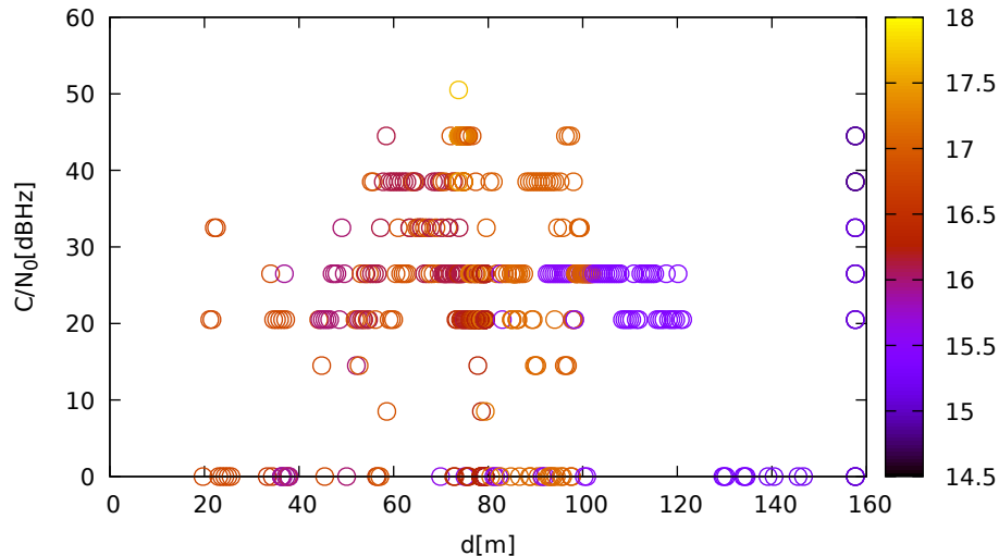
C/N 0 vs distance (LeicaGS18 at C 2 for G28 at L1)
