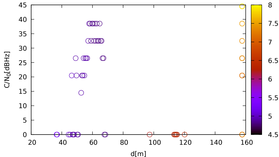
C/N 0 vs distance (LeicaGS18 at C 2 for G31 at L1)
