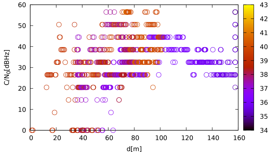
C/N 0 vs distance (LeicaGS18 at C 2 for G32 at L1)
