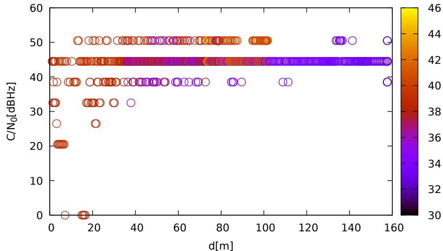
C/N 0 vs distance (LeicaGS18 at C 2 for R06 at L1)
