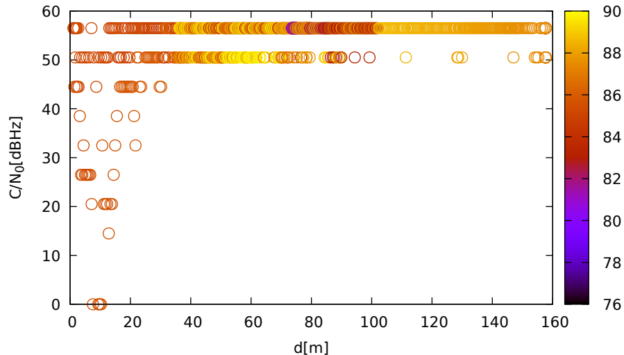
C/N 0 vs distance (LeicaGS18 at C 2 for R07 at L1)
