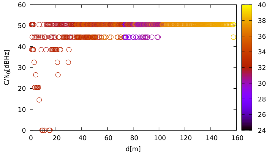
C/N 0 vs distance (LeicaGS18 at C 2 for R08 at L1)
