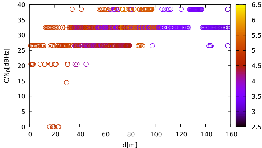
C/N 0 vs distance (LeicaGS18 at C 2 for R14 at L1)
