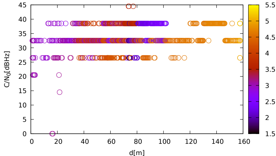
C/N 0 vs distance (LeicaGS18 at C 2 for R15 at L1)
