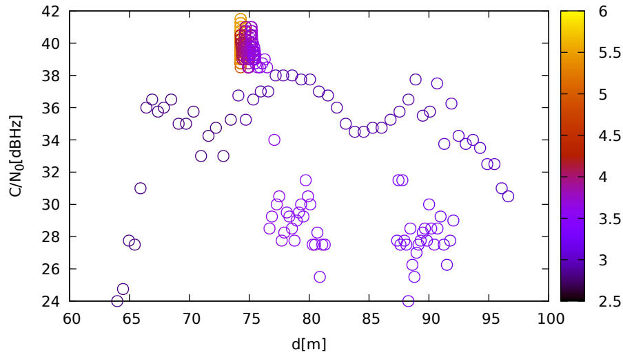
C/N 0 vs distance (TrimbleR10 at C 2 for E02 at L1)
