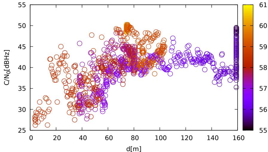
C/N 0 vs distance (TrimbleR10 at C 2 for E04 at L1)
