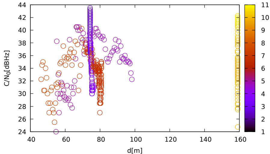
C/N 0 vs distance (TrimbleR10 at C 2 for E05 at L1)
