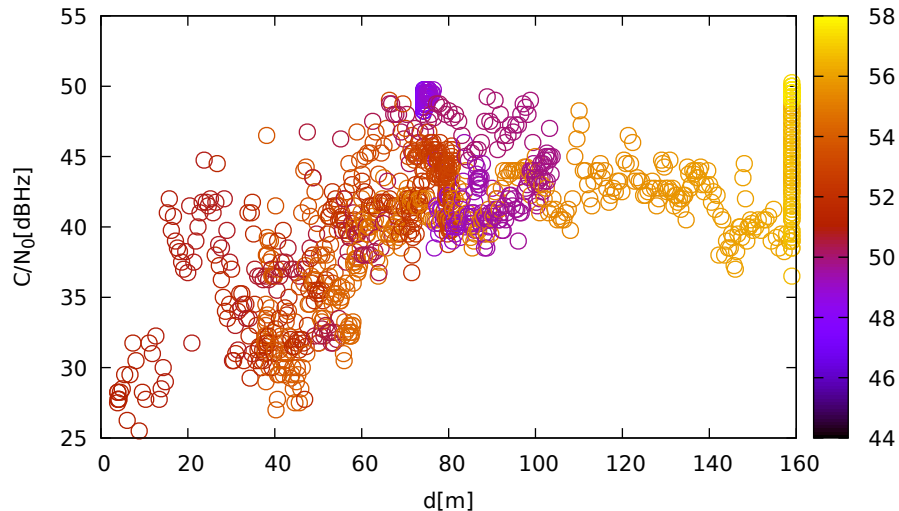
C/N 0 vs distance (TrimbleR10 at C 2 for E09 at L1)
