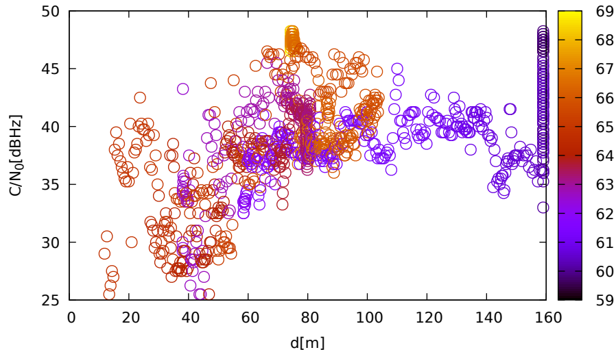
C/N 0 vs distance (TrimbleR10 at C 2 for E11 at L1)
