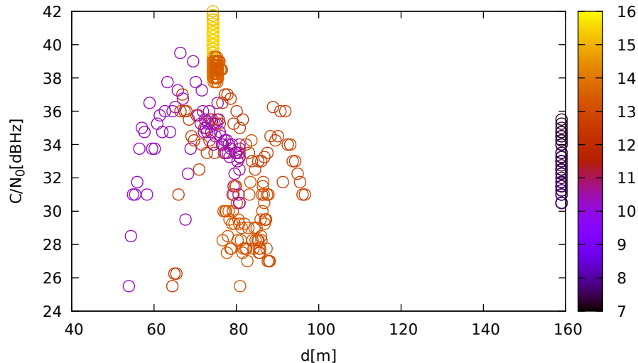
C/N 0 vs distance (TrimbleR10 at C 2 for E12 at L1)
