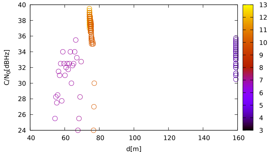
C/N 0 vs distance (TrimbleR10 at C 2 for E19 at L1)
