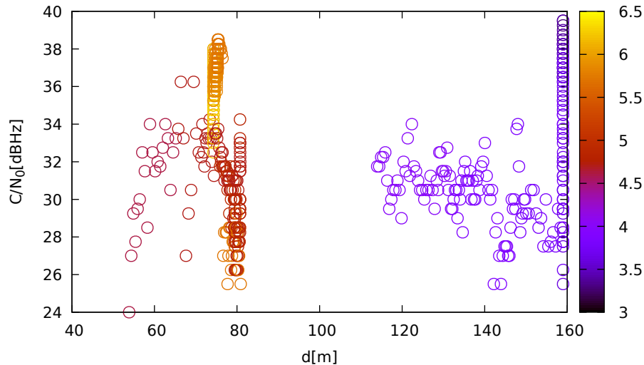
C/N 0 vs distance (TrimbleR10 at C 2 for E30 at L1)
