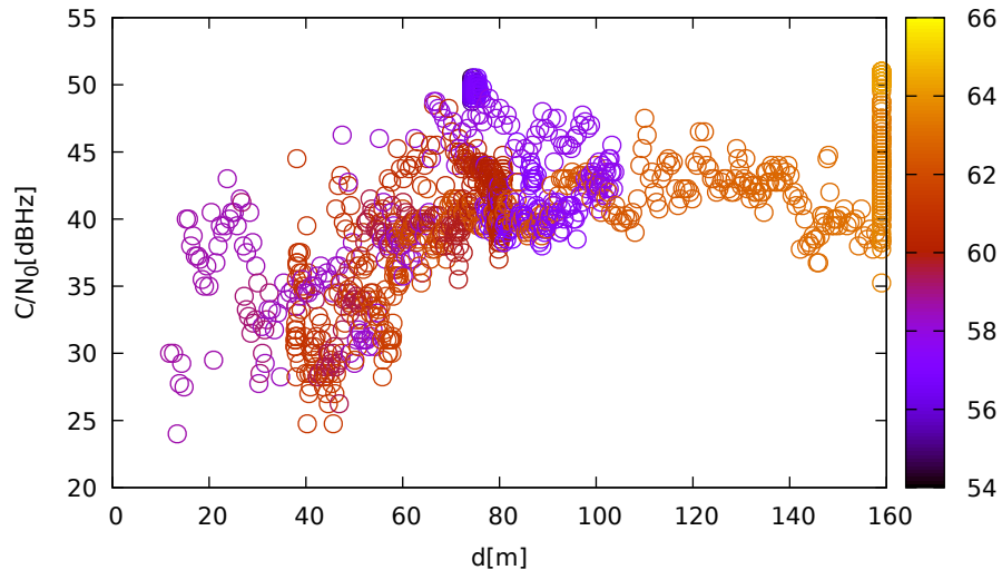
C/N 0 vs distance (TrimbleR10 at C 2 for E36 at L1)
