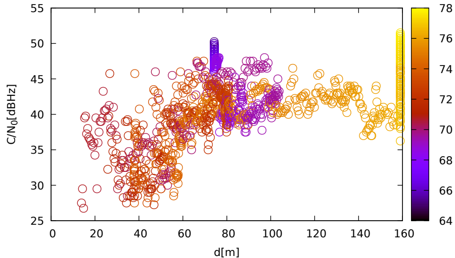
C/N 0 vs distance (TrimbleR10 at C 2 for G01 at L1)
