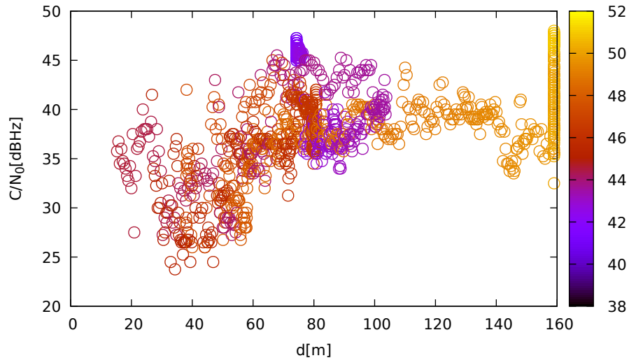
C/N 0 vs distance (TrimbleR10 at C 2 for G03 at L1)
