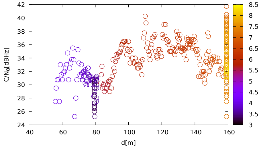
C/N 0 vs distance (TrimbleR10 at C 2 for G04 at L1)
