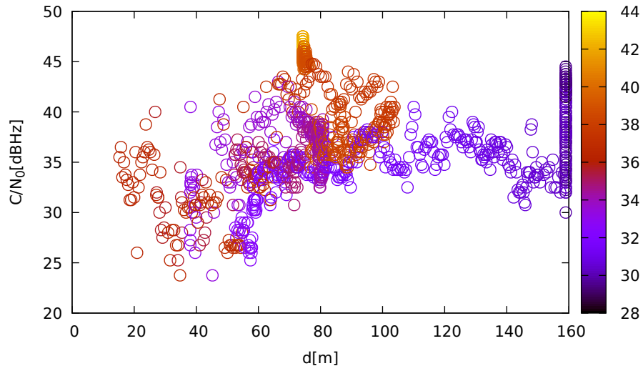
C/N 0 vs distance (TrimbleR10 at C 2 for G08 at L1)
