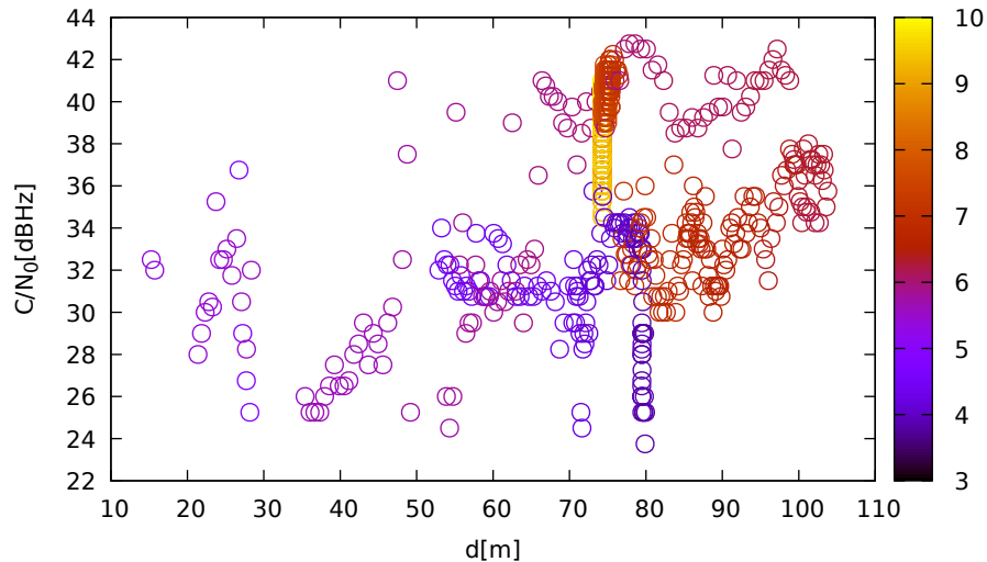
C/N 0 vs distance (TrimbleR10 at C 2 for G10 at L1)
