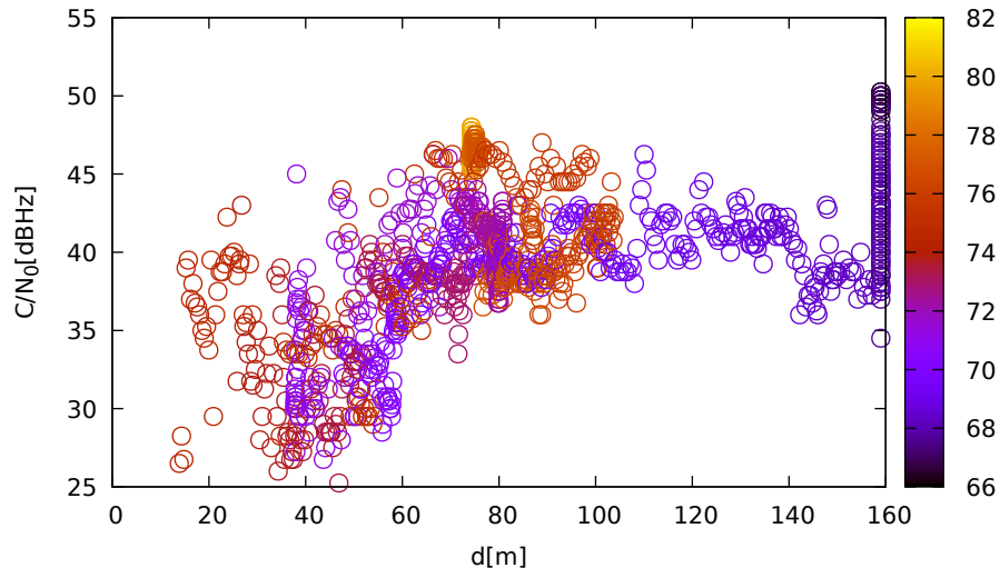
C/N 0 vs distance (TrimbleR10 at C 2 for G11 at L1)
