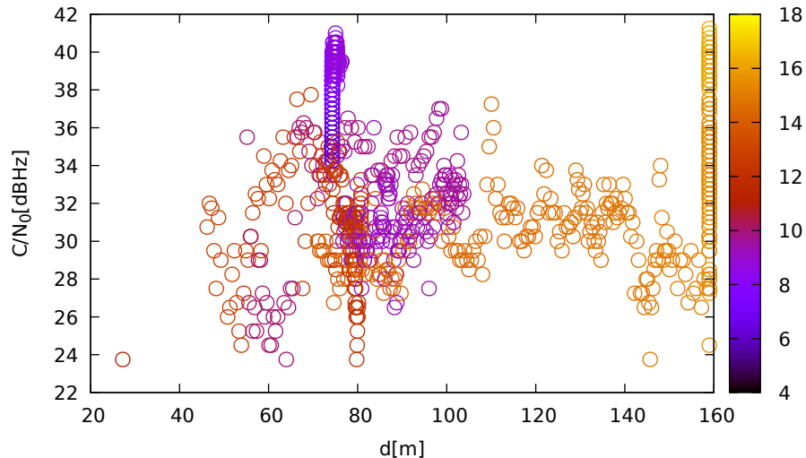
C/N 0 vs distance (TrimbleR10 at C 2 for G17 at L1)
