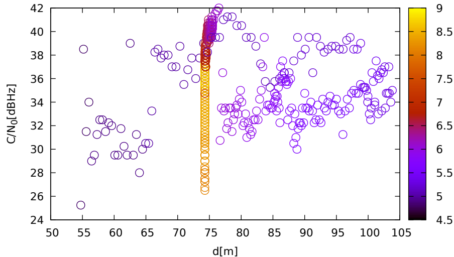
C/N 0 vs distance (TrimbleR10 at C 2 for G21 at L1)
