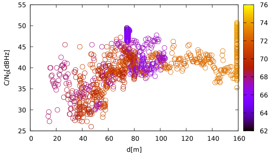
C/N 0 vs distance (TrimbleR10 at C 2 for G22 at L1)
