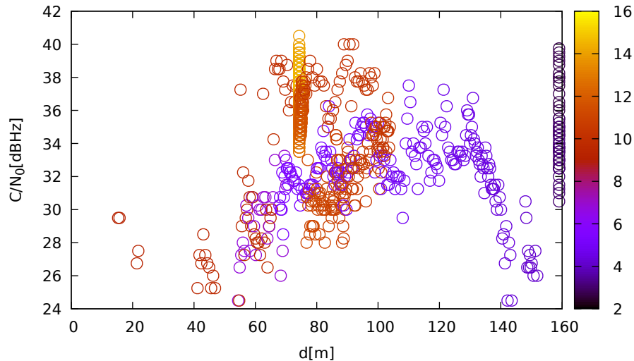
C/N 0 vs distance (TrimbleR10 at C 2 for G27 at L1)
