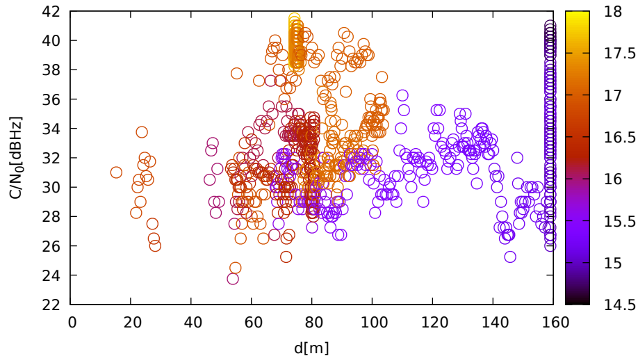
C/N 0 vs distance (TrimbleR10 at C 2 for G28 at L1)
