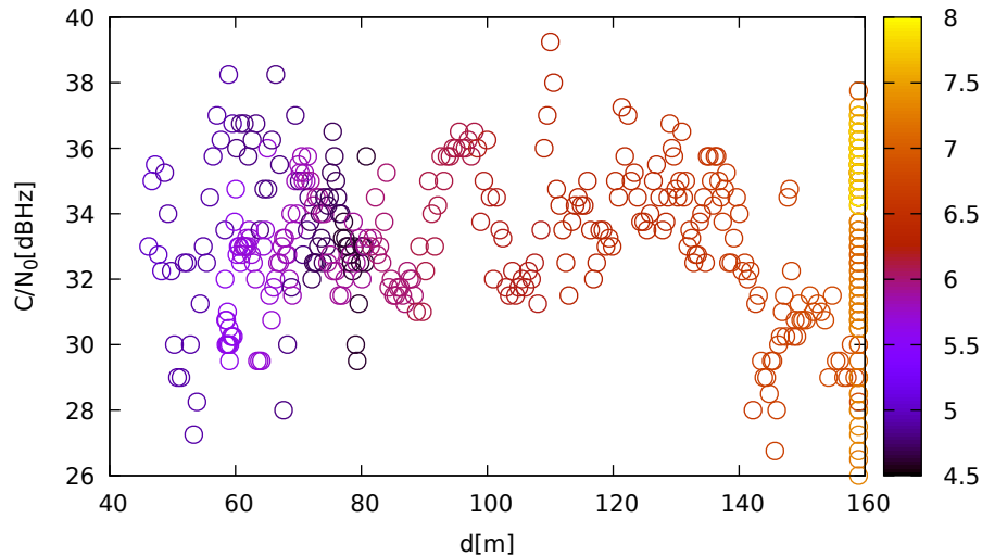
C/N 0 vs distance (TrimbleR10 at C 2 for G31 at L1)
